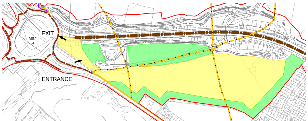
Insert 2 Site Compound (extract from TR010034/APP/2.8 Temporary Works Plan)
